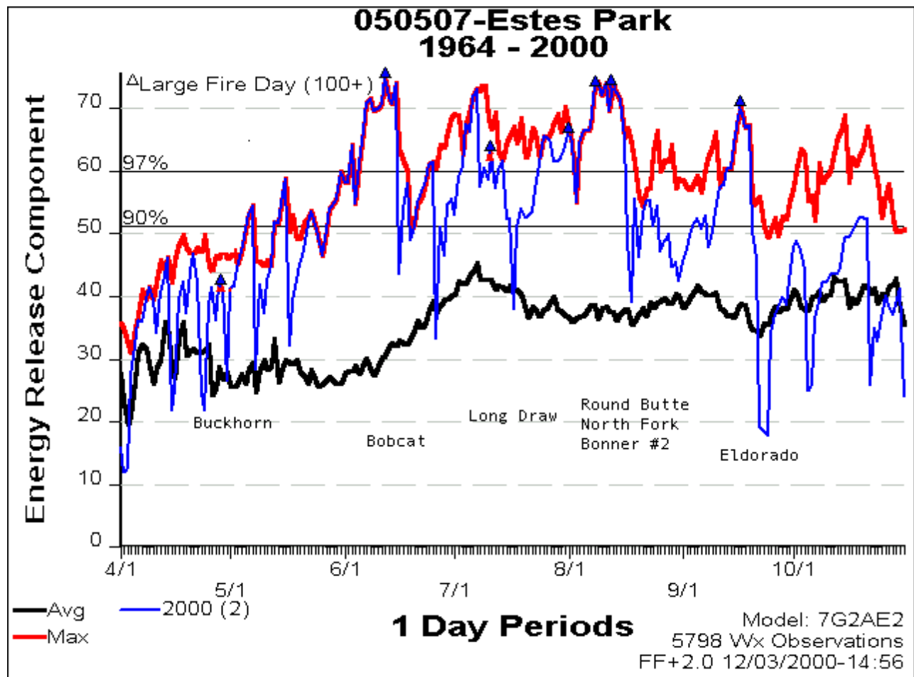
2000 seasonal ERC chart for the Estes Park weather station
